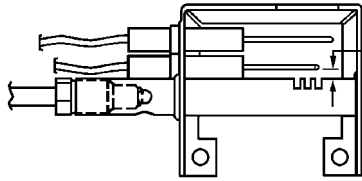
Horizontal Burner with Sense Electrode
