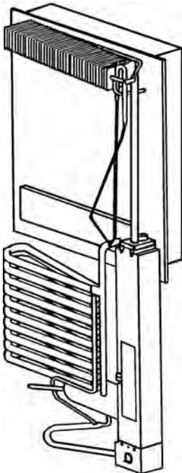
Cooling Unit
