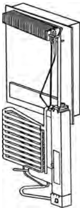
Cooling Unit
