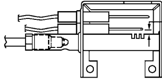
Horizontal Burner with Sense Electrode
